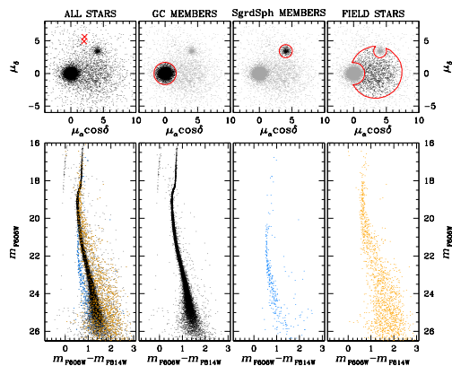
Fig. 1. Top panels : proper-motion diagrams in the core of the GC NGC 6681. From left to right: all measured sources (red crosses mark the location of 2 galaxies in the field); selected cluster members, selected Sgr dSph members, and field stars. Bottom panels : CMDs for all sources, GC members (black), Sgr dSph members (azure), and field stars (yellow).
