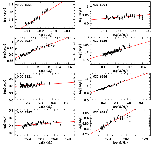
Fig. 4. Average velocity dispersion vs. Mass for a sample of 8 clusters, in the log-log plane. The scale ratio of the axes is the same in all panels. It is clear that the power-law relation between average velocity dispersion and stellar mass does not have a universal slope.
