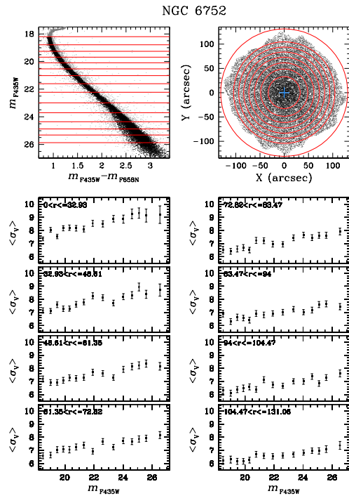
Fig. 2. Velocity-dispersion analysis for NGC 6752. Top panels show the selection of main-sequence stars in bins of magnitude (left) and radial distance from the cluster center (right). In the bottom panels, for each radial interval we plot the average velocity dispersion as a function of the magnitude.
