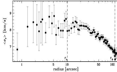
Fig. 3. \langle \sigma_V \rangle as a function of the radial distance for all NGC 6752 stars in the field.
